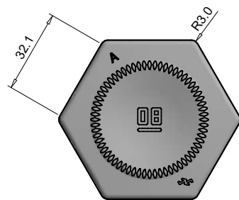
VIEW OF BASE SHOWING EMBOSSING MARKINGS & STACKING RING EMBOSSED WITH STIPPLES
