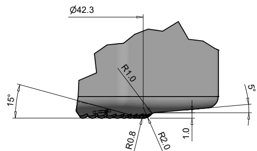
(3 : 1) STACKING RING DETAIL
