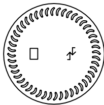
VIEW ON BASE SHOWING EMBOSSED MARKING STANDING AREA EMBOSSED WITH CRESCENT STIPPLE
